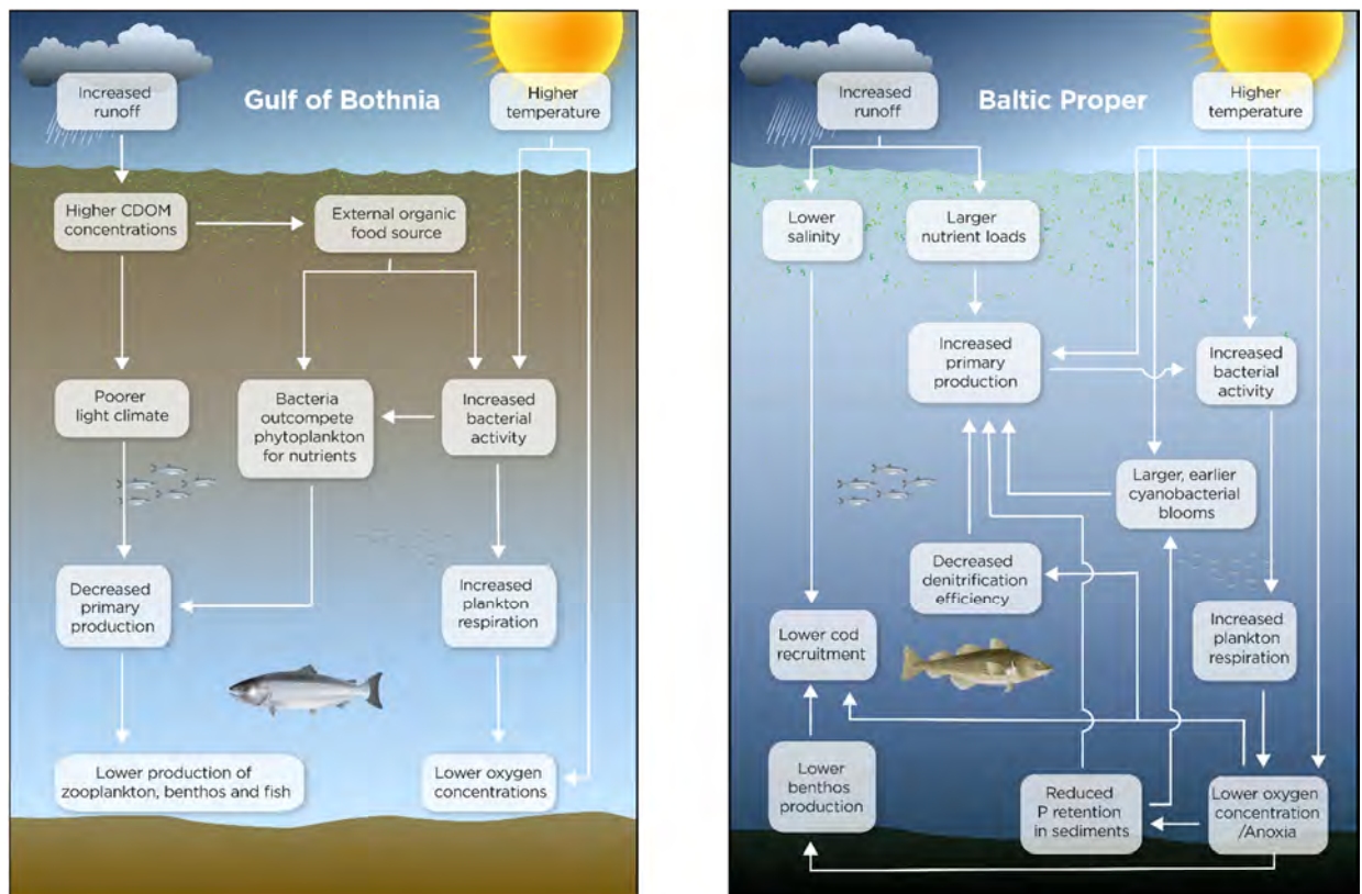
Figure 1. General characteristics of the Gulf of Bothnia and the Baltic Proper.
